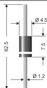
Axial lead diode
