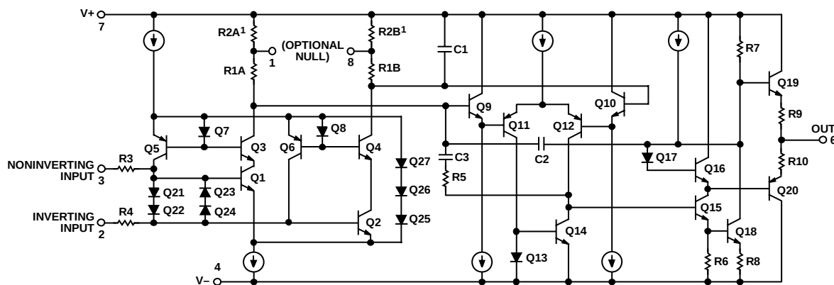
Figure 2. Simplified Schematic
