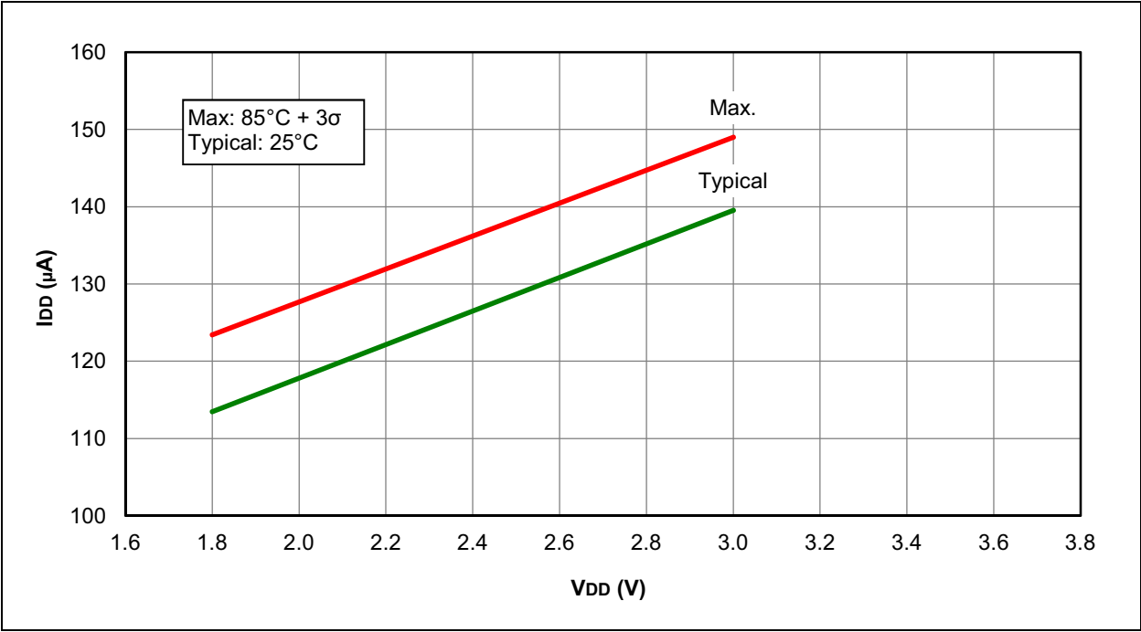
FIGURE 31-13: I DD , MFINTOSC MODE (F osc = 500 kHz), PIC16LF1824/1828 ONLY
