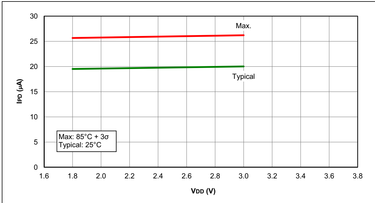
FIGURE 31-39: I_{PD} , COMPARATOR, NORMAL-POWER MODE ( CxSP = 1 ), PIC16LF1824/1828 ONLY
