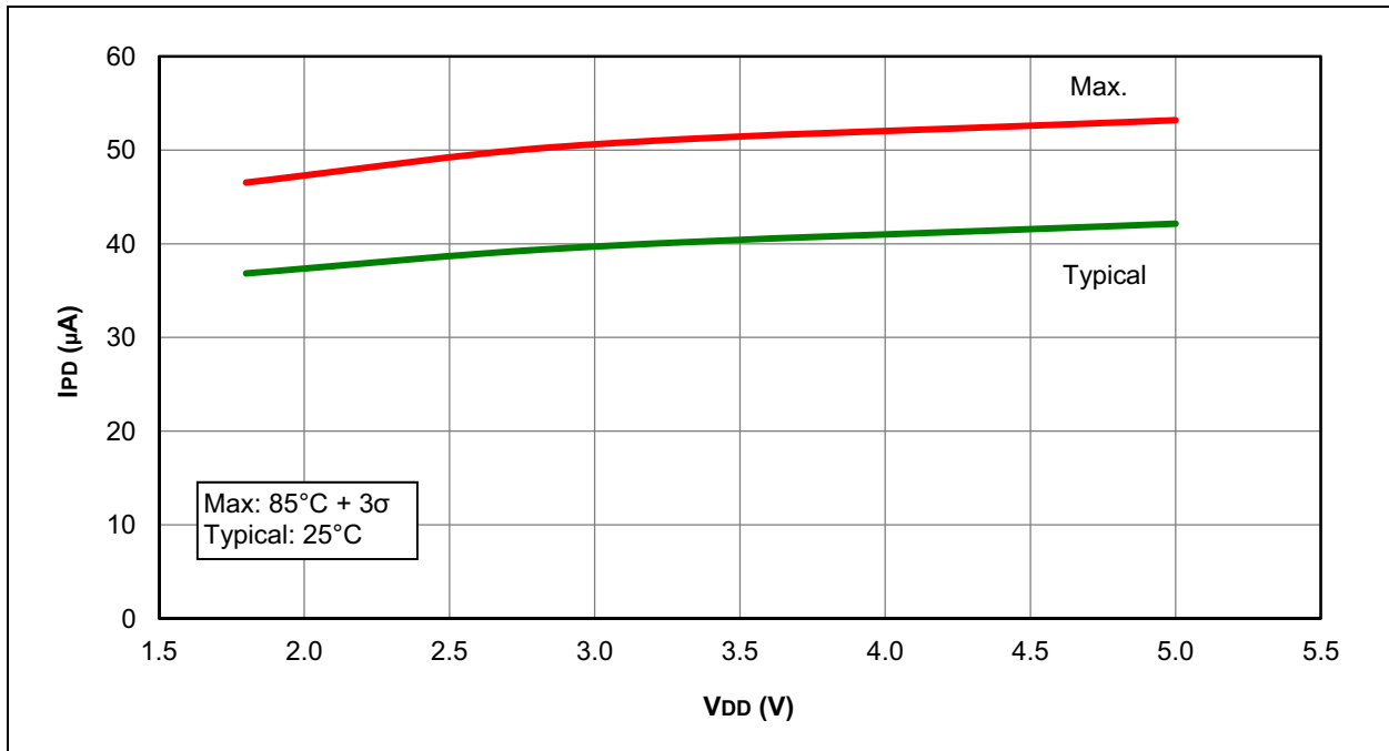
FIGURE 31-40: I_{PD} , COMPARATOR, NORMAL-POWER MODE ( CxSP = 1 ), PIC16F1824/1828 ONLY
