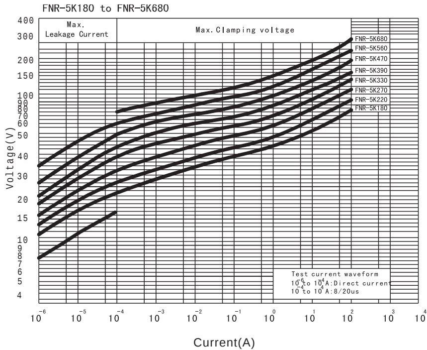
V-I Curve
