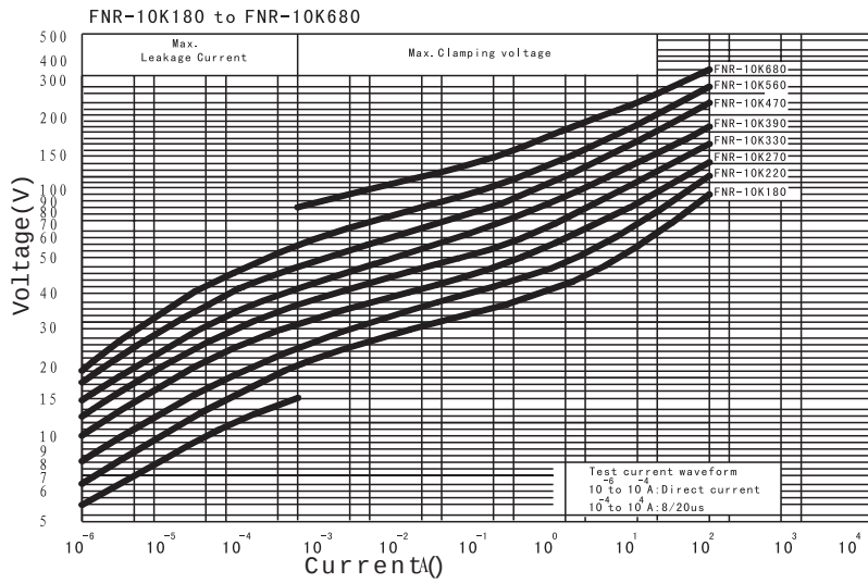
V-I Curve
