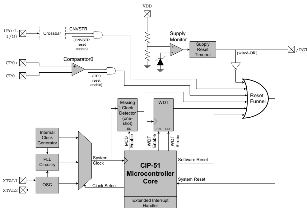
Figure 14.1. Reset Sources
