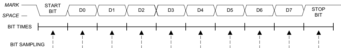
Figure 22.4. UART0 Mode 1 Timing Diagram
