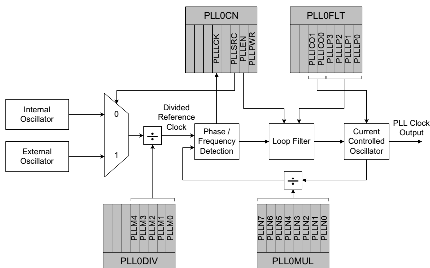
Figure 15.6. PLL Block Diagram
