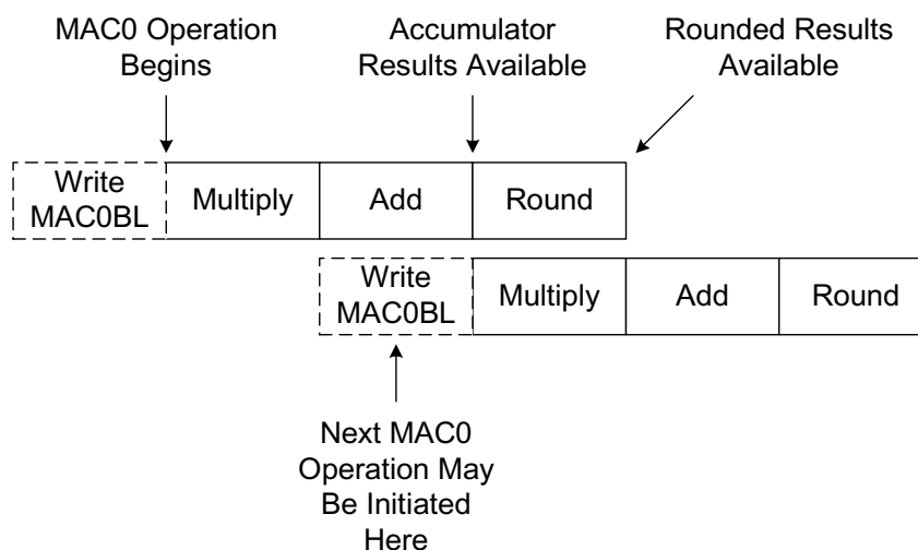
Figure 13.4. MAC0 Pipeline
