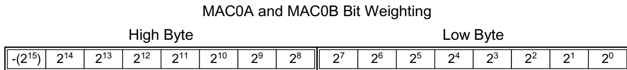
Figure 13.2. Integer Mode Data Representation
