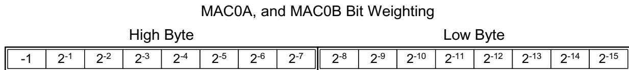
Figure 13.3. Fractional Mode Data Representation
