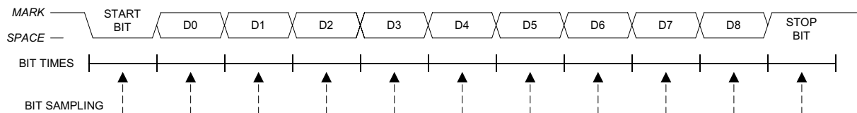
Figure 22.5. UART0 Modes 2 and 3 Timing Diagram
