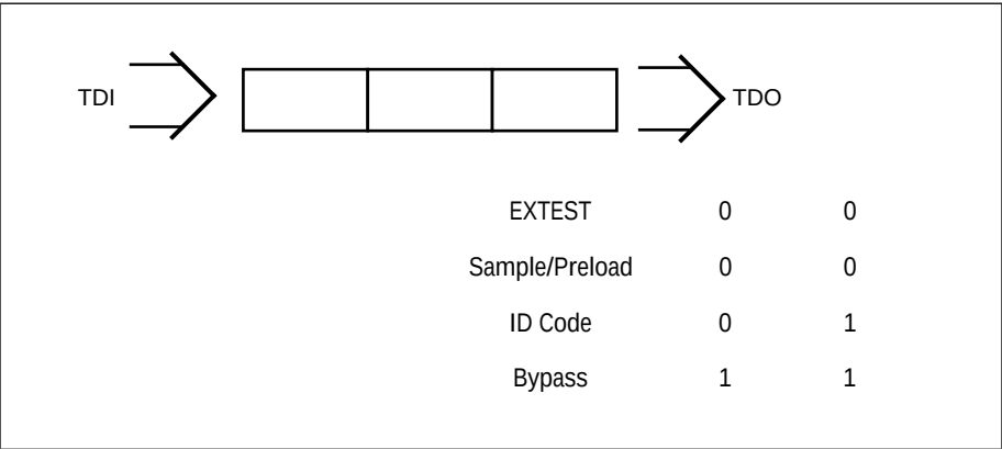
Figure 2-16. Instruction Register
