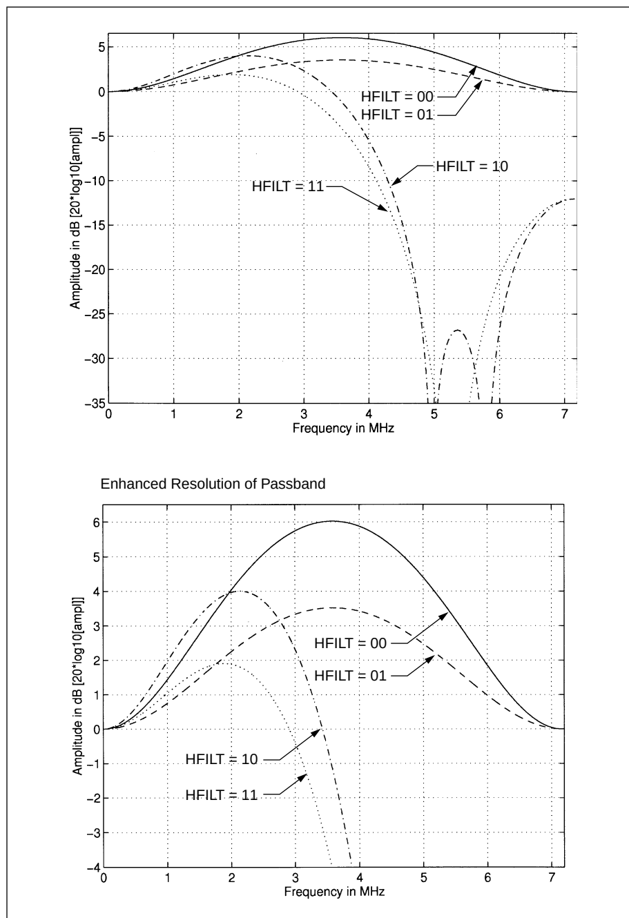
Figure 1-12. Peaking Filters
