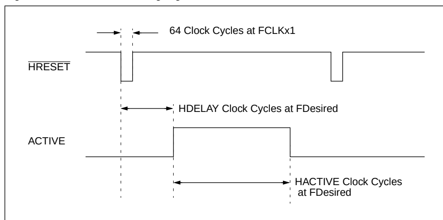
Figure 2-12. Horizontal Timing Signals in the SPI Modes
