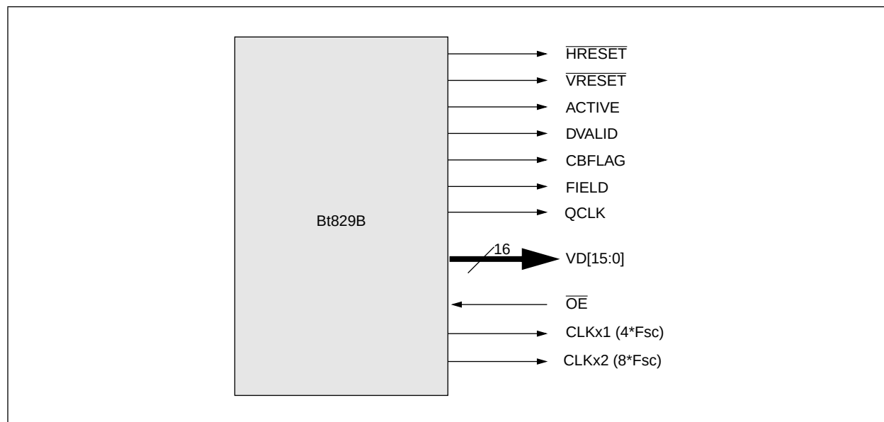
Figure 2-8. Bt829B/827B Synchronous Pixel Interface, Mode 1 (SPI-1)
