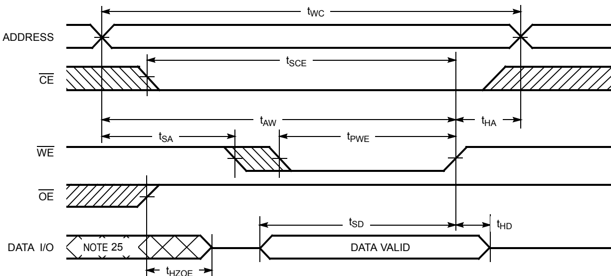
Figure 9. Write Cycle No. 1 ( \overline{\text{WE}} controlled) [21, 22, 23, 24]
