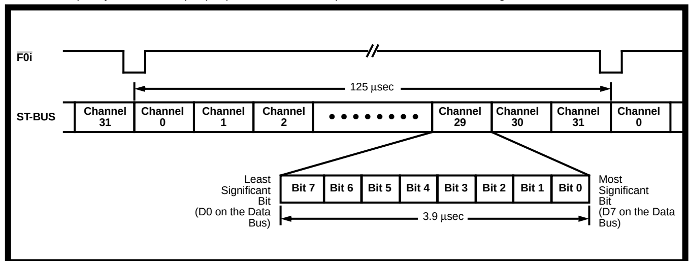
Figure 24 - ST-BUS Format
