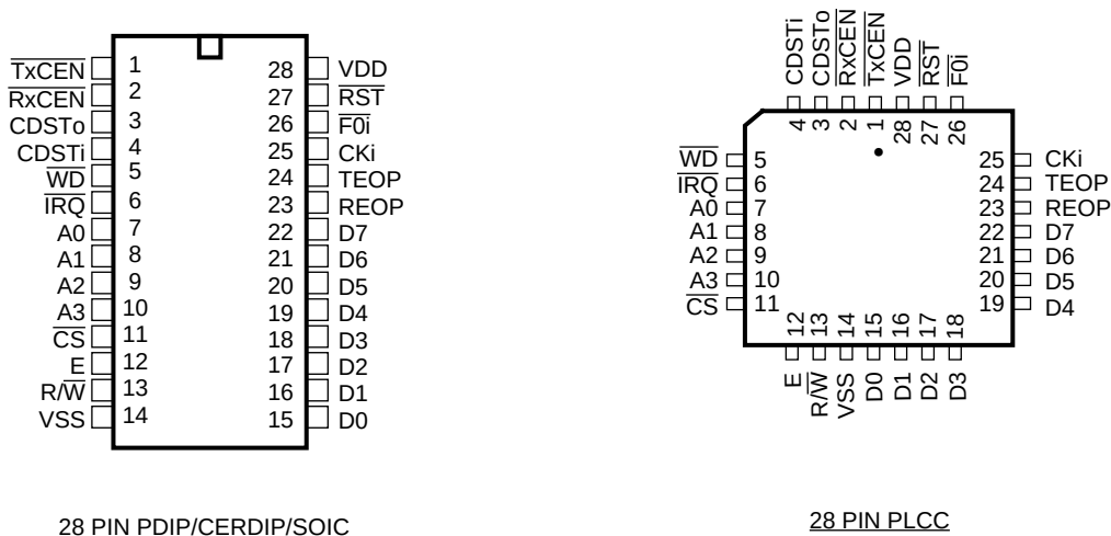
Figure 2 - Pin Connections
