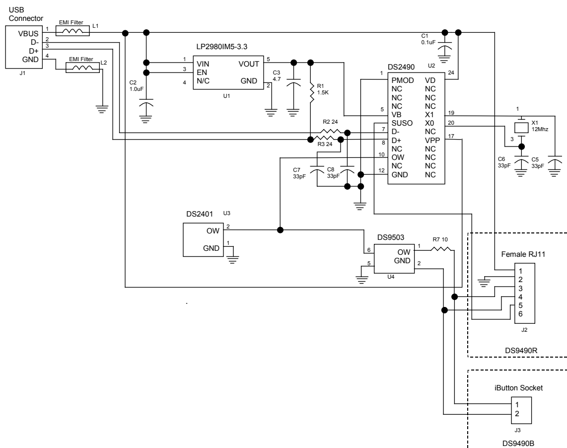
Figure 8. FUNCTIONAL DIAGRAM
