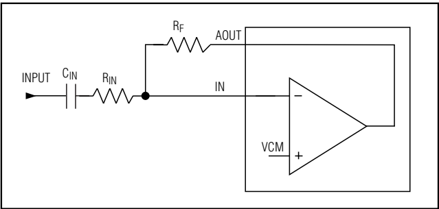
Figure 3. Input Amplifier Configuration
