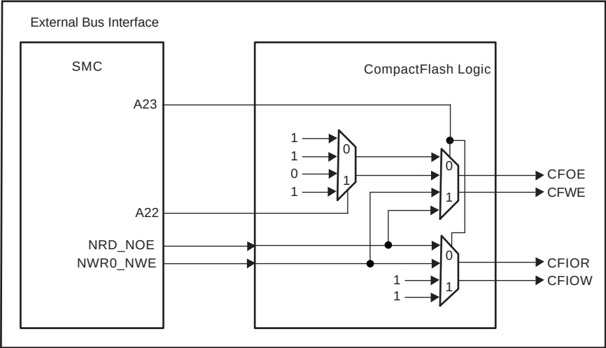
Figure 19-6. CompactFlash Read/Write Control Signals
