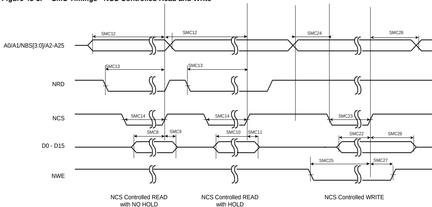
Figure 45-3. SMC Timings - NCS Controlled Read and Write
