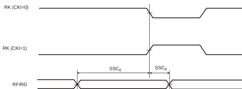
Figure 45-14. SSC Receiver RK and RF in Input
