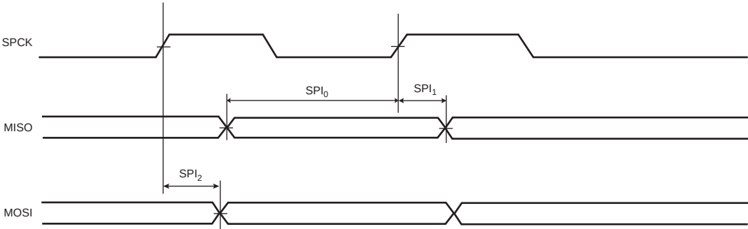
Figure 45-5. SPI Master Mode 1 and 2
