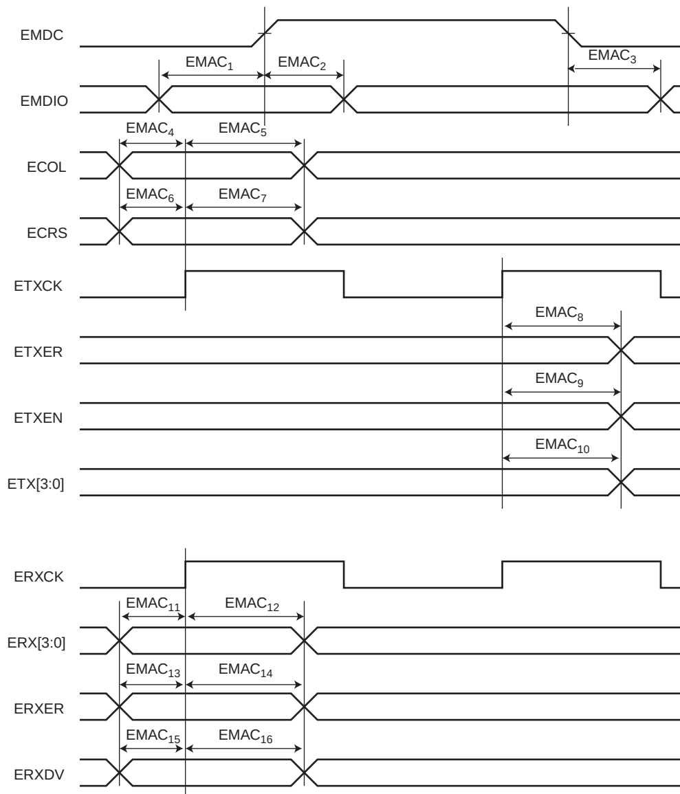
Figure 45-21. EMAC MII Mode
