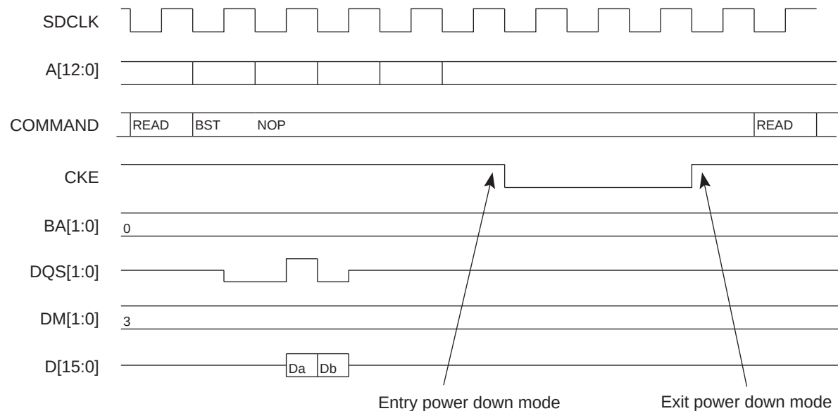
Figure 21-22. Power-down Entry/Exit, Timeout = 0
