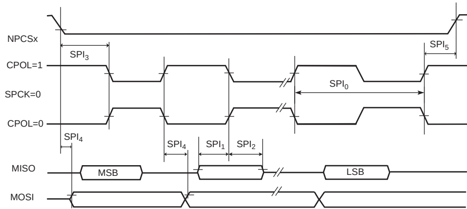
Figure 45-23. UART SPI Master Mode
