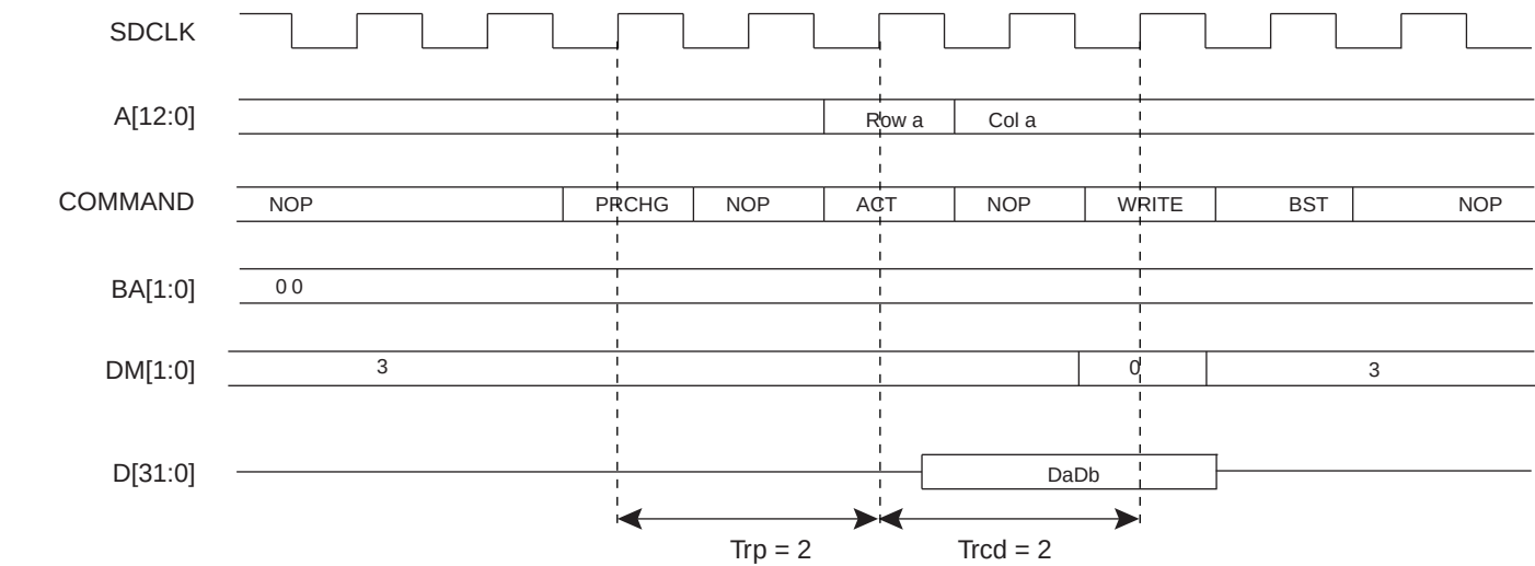
Figure 21-4. Single Write Access, Row Closed, SDR-SDRAM Device
