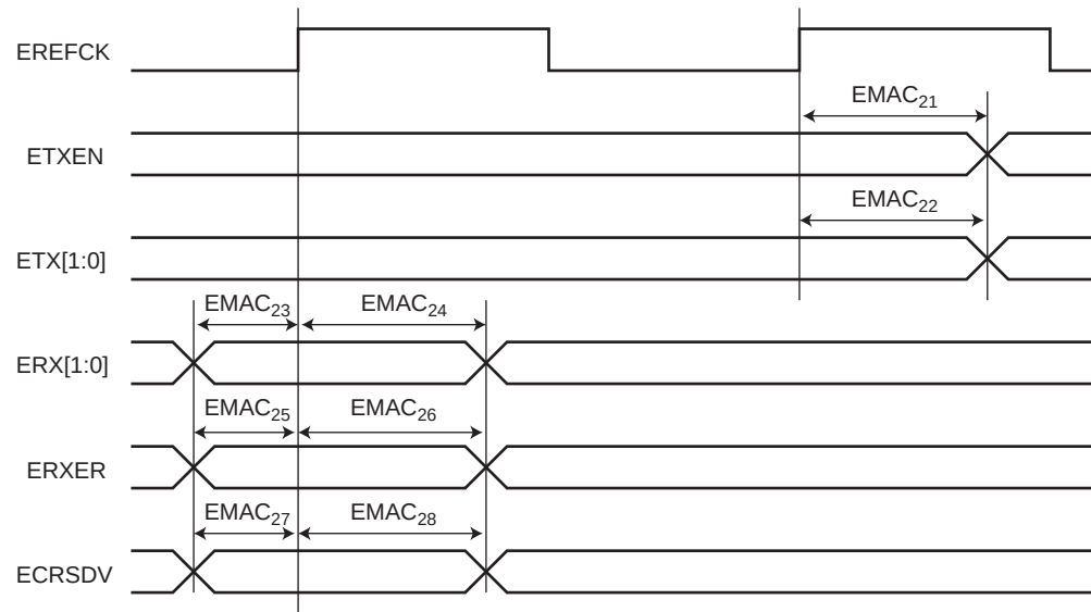
Figure 45-22. EMAC RMII Timings
