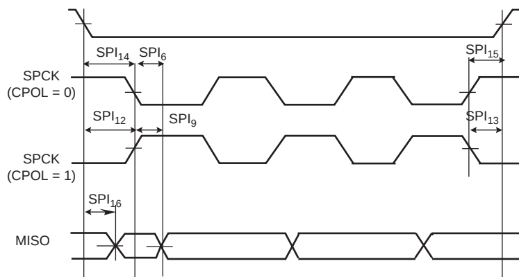
Figure 45-25. SPI Slave Mode - NPCS Timings
