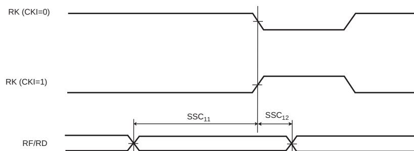
Figure 45-17. SSC Receiver, RK in Output and RF in Input
