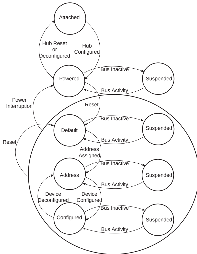
Figure 37-19. UDPSH Device State Diagram
