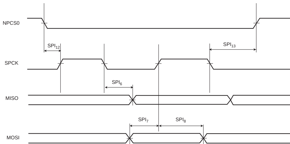
Figure 45-24. UART SPI Slave Mode
