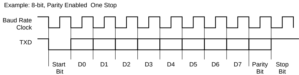
Figure 32-6. Character Transmit
