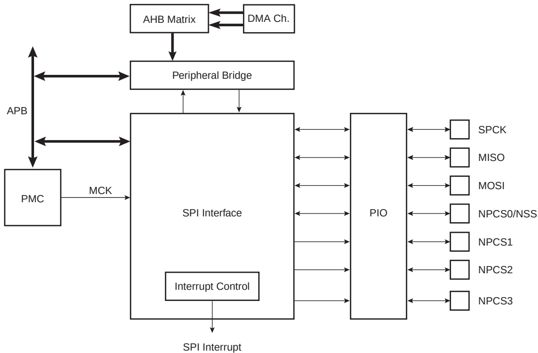
Figure 28-1. Block Diagram
