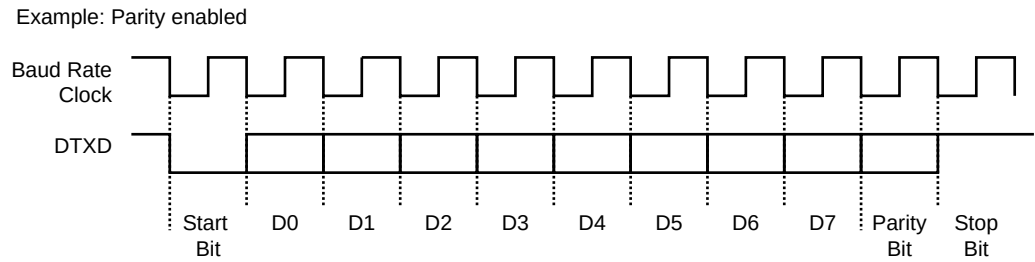
Figure 27-10. Character Transmission
