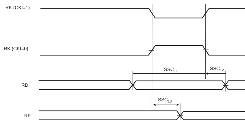
Figure 45-16. SSC Receiver, RK and RF in Output
