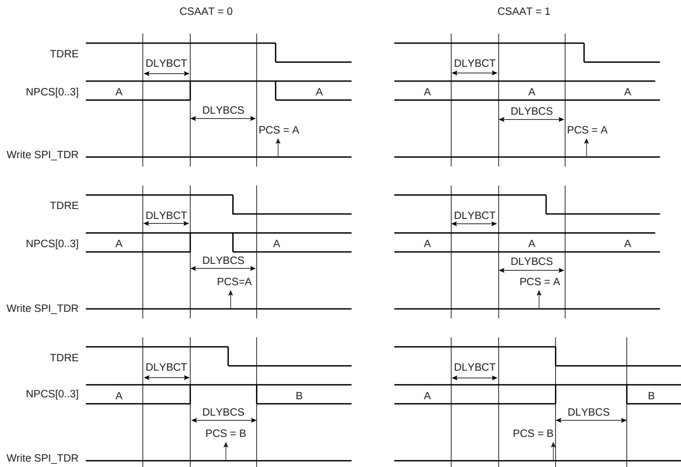
Figure 28-10. Peripheral Deselection
