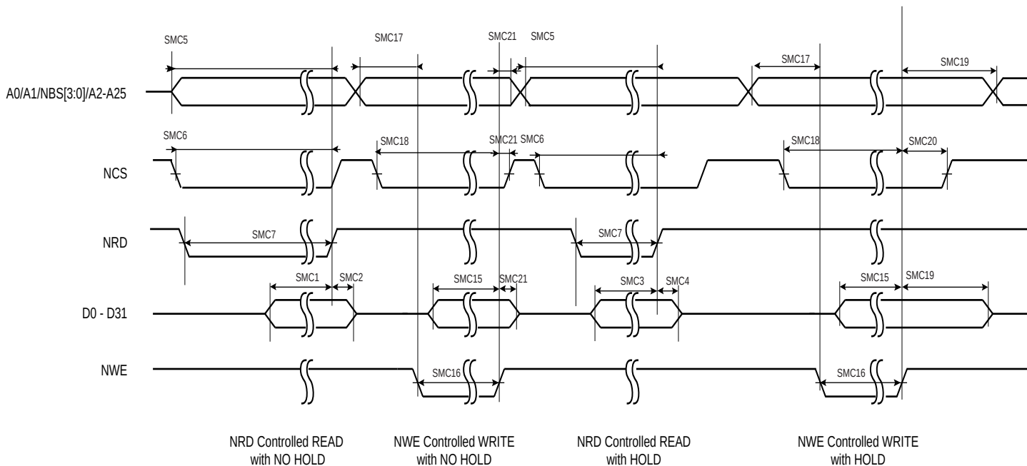
Figure 45-4. SMC Timings - NRD Controlled Read and NWE Controlled Write
