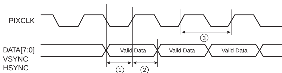
Figure 45-19. ISI Timing Diagram
