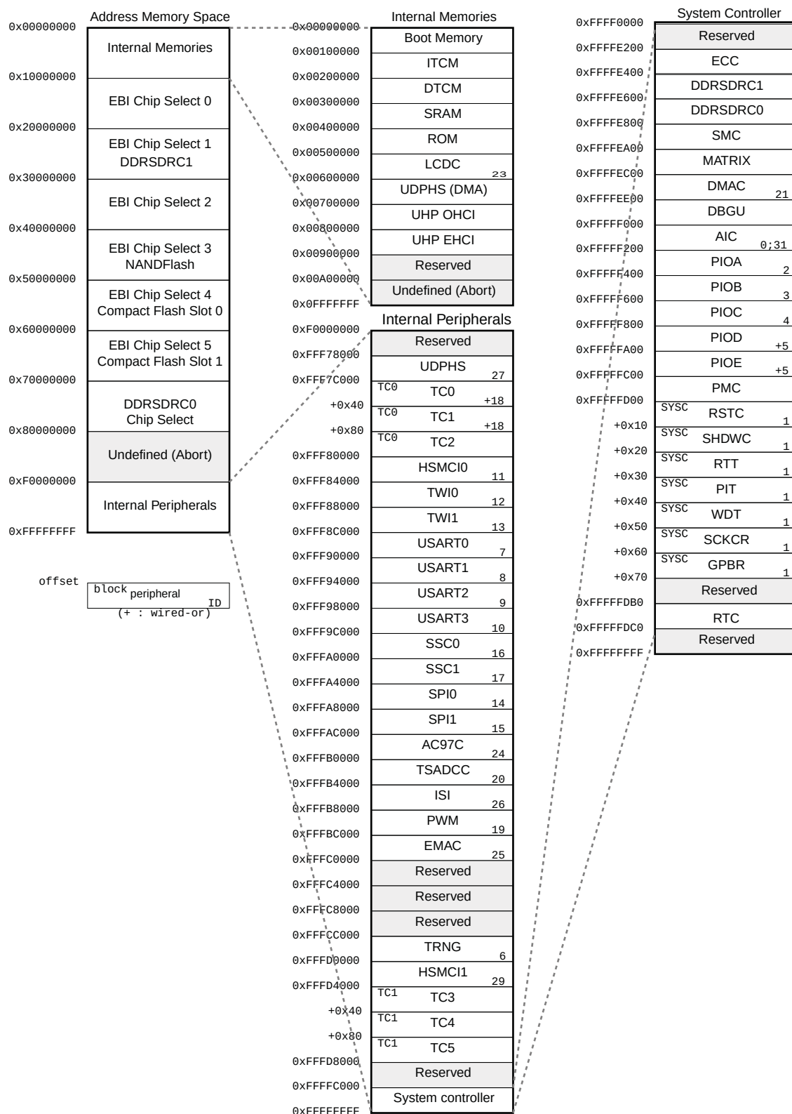
Figure 5-1. SAM9G45 Memory Mapping
