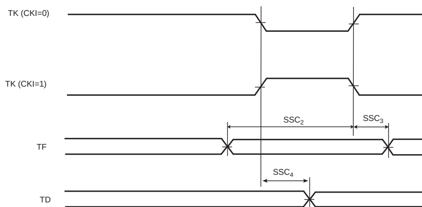
Figure 45-13. SSC Transmitter, TK in Output and TF in Input
