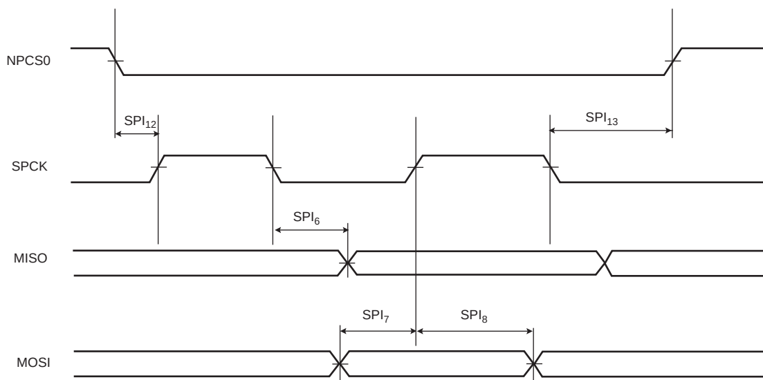
Figure 45-7. SPI Slave Mode 0 and 3)
