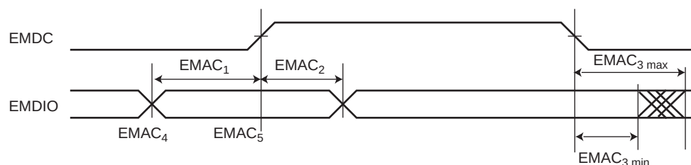
Figure 45-20. Min and Max Access Time of EMAC Output Signals
