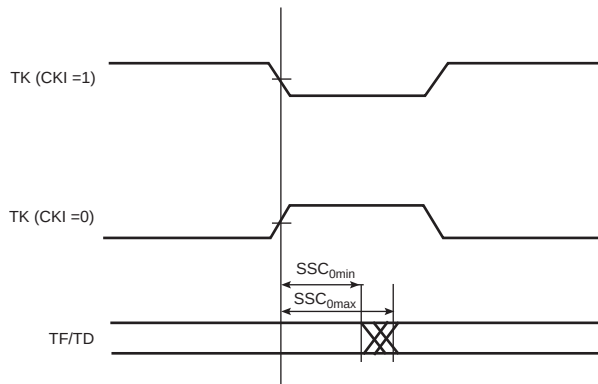
Figure 45-18. Min and Max Access Time of Output Signals
