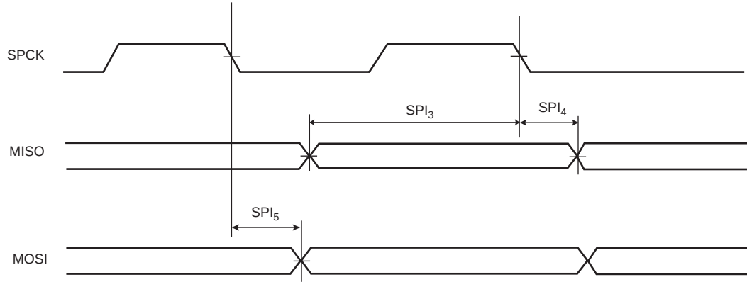
Figure 45-6. SPI Master Mode 0 and 3
