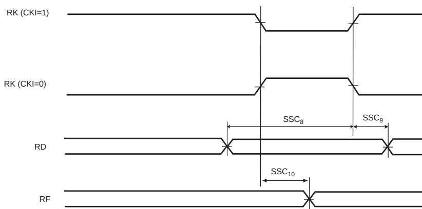
Figure 45-15. SSC Receiver, RK in Input and RF in Output
