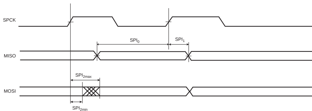
Figure 45-10. Min and Max Access Time for SPI Output Signal
