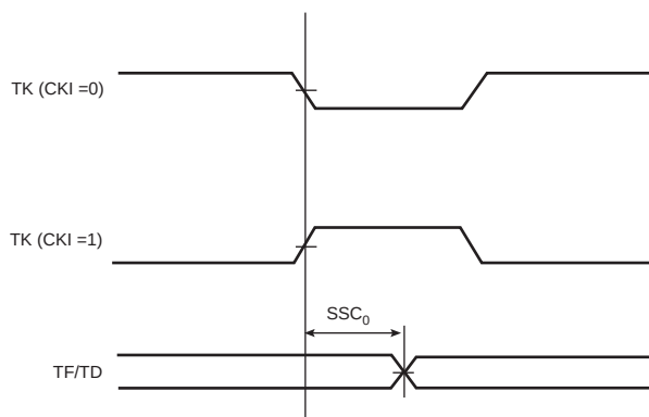
Figure 45-11. SSC Transmitter, TK and TF in Output
