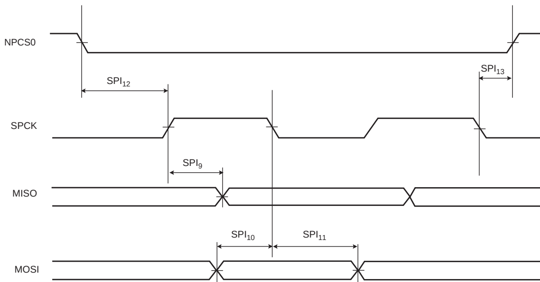
Figure 45-8. SPI Slave Mode 1 and 2
