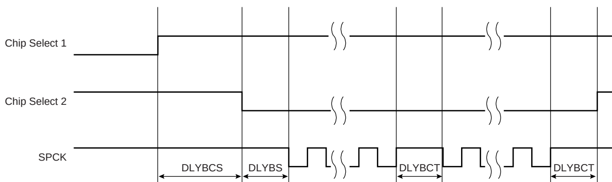
Figure 28-8. Programmable Delays
