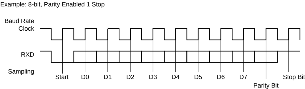
Figure 32-20. Synchronous Mode Character Reception
