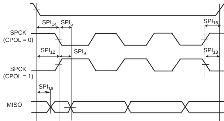
Figure 45-9. SPI Slave Mode - NPCS Timings
