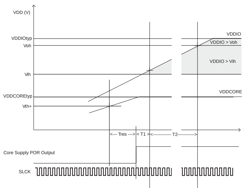
Figure 45-2. VDDCORE and VDDIO Constraints at Startup
