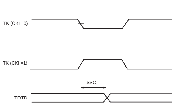
Figure 45-12. SSC Transmitter, TK in Input and TF in Output
